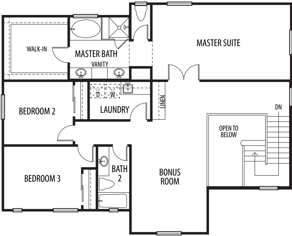
2ND FLOOR
